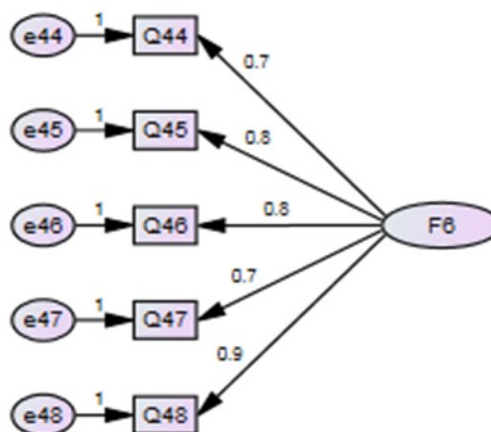
Figure 6) Factor loads of over-identification
